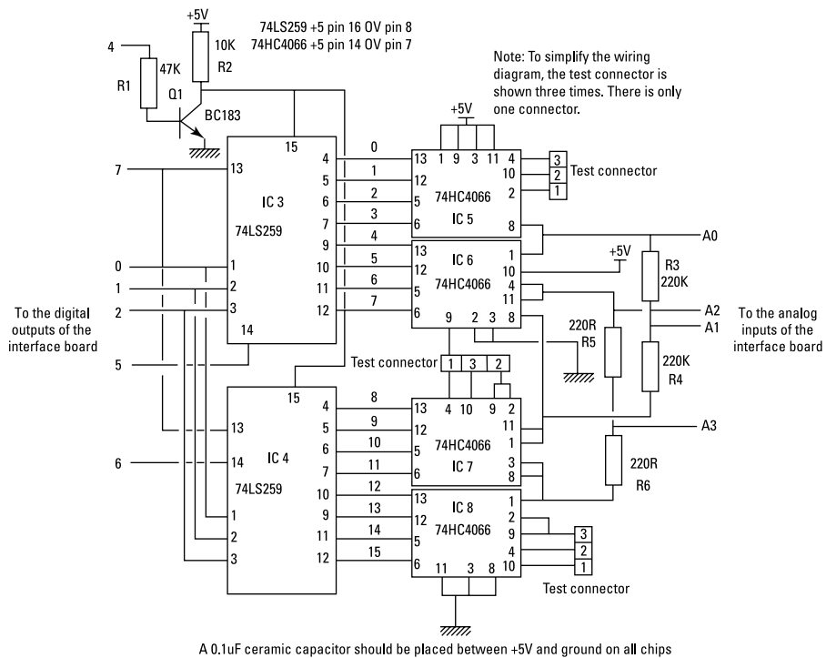
Figure 18-9: Test circuit schematic.
