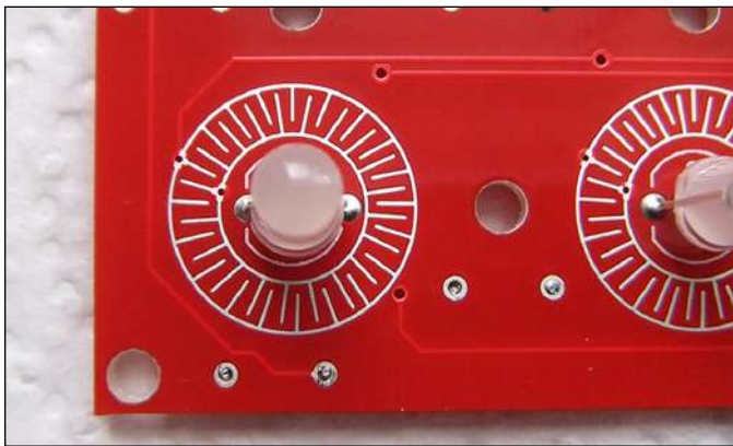
Figure 7-9: The mounting of the LEDs.
