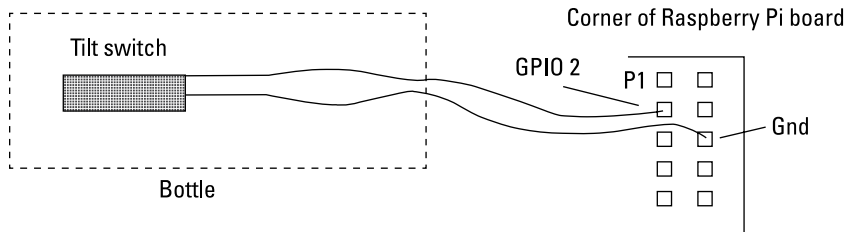
Figure 5-2: The sauce bottle schematic.
